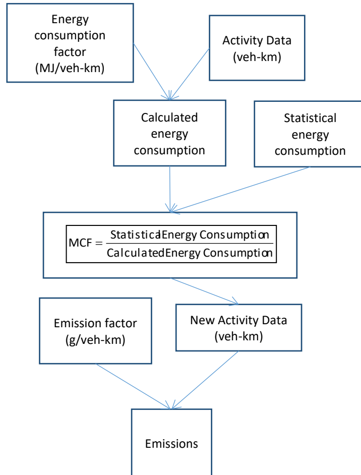
Figure 3-3: Flow chart of the fuel energy balance algorithm
