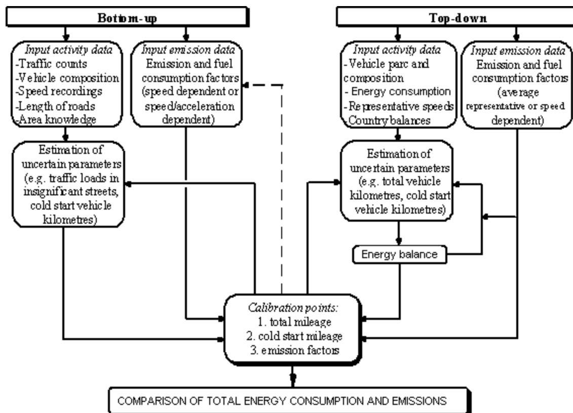
Figure 4-1: Proposed reconciliation method in applying bottom-up and top-down approaches when building an urban emission inventory
